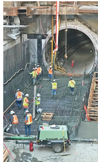
L.A. Metro Station Alameda & 1st Streets Project for contractor Skanska: Concrete slab pour in progress (above), funny trowling / hand trowling, (upper right), Journeyman & Job Steward Jose Muniz hard trowling (right).
