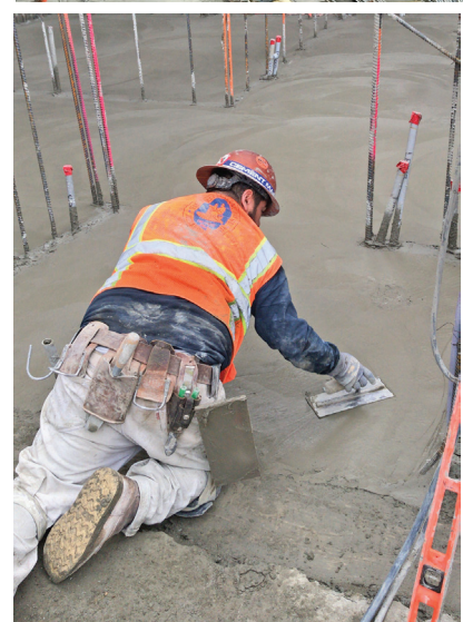
L.A. Metro Station Alameda & 1st Streets Project for contractor Skanska: Concrete slab pour in progress (above), funny trowling / hand trowling, (upper right), Journeyman & Job Steward Jose Muniz hard trowling (right).
